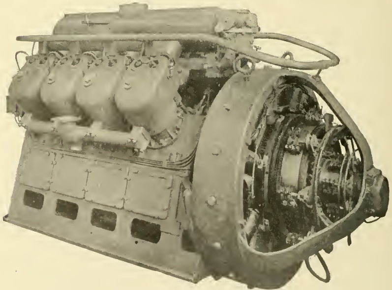
Fig. 14. Gas Engine and Generator of Gas-Electric Car.
